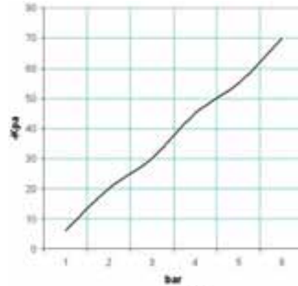
Air consumption (Nm/s) at different supply pressures (bar)
